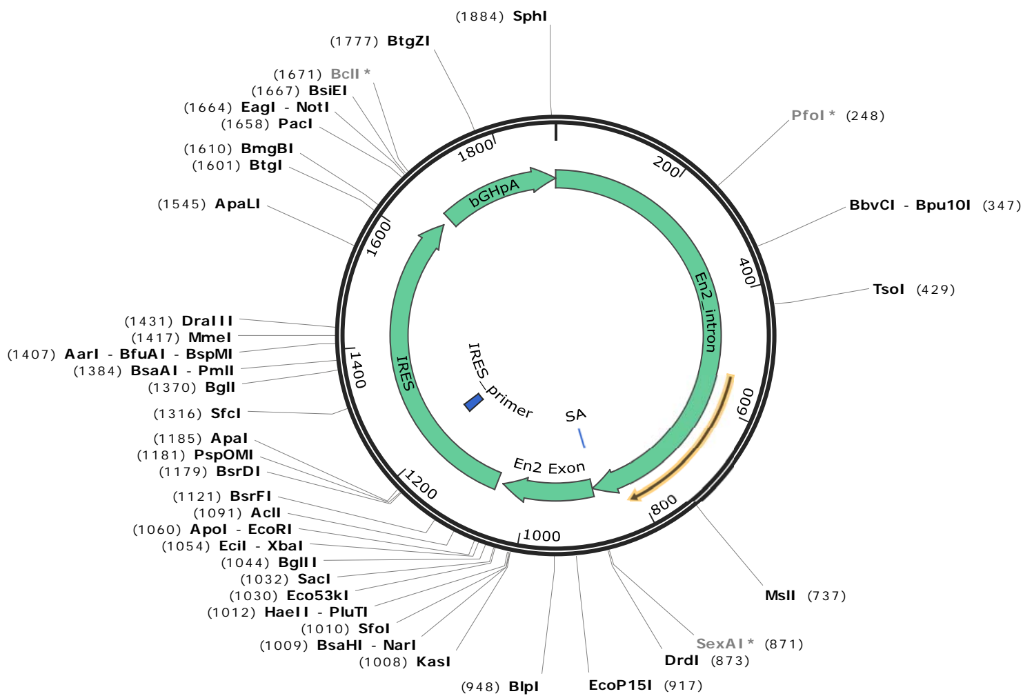
En2_IRES_CREERT2_bGHpA 1891 bp
